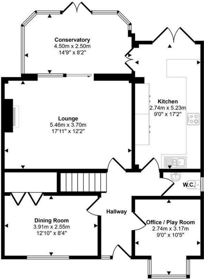
Ground Floor Approx 79 sq m / 849 sq ft
